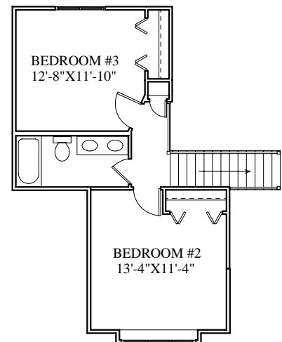
UPPER LEVEL FLOOR PLAN
