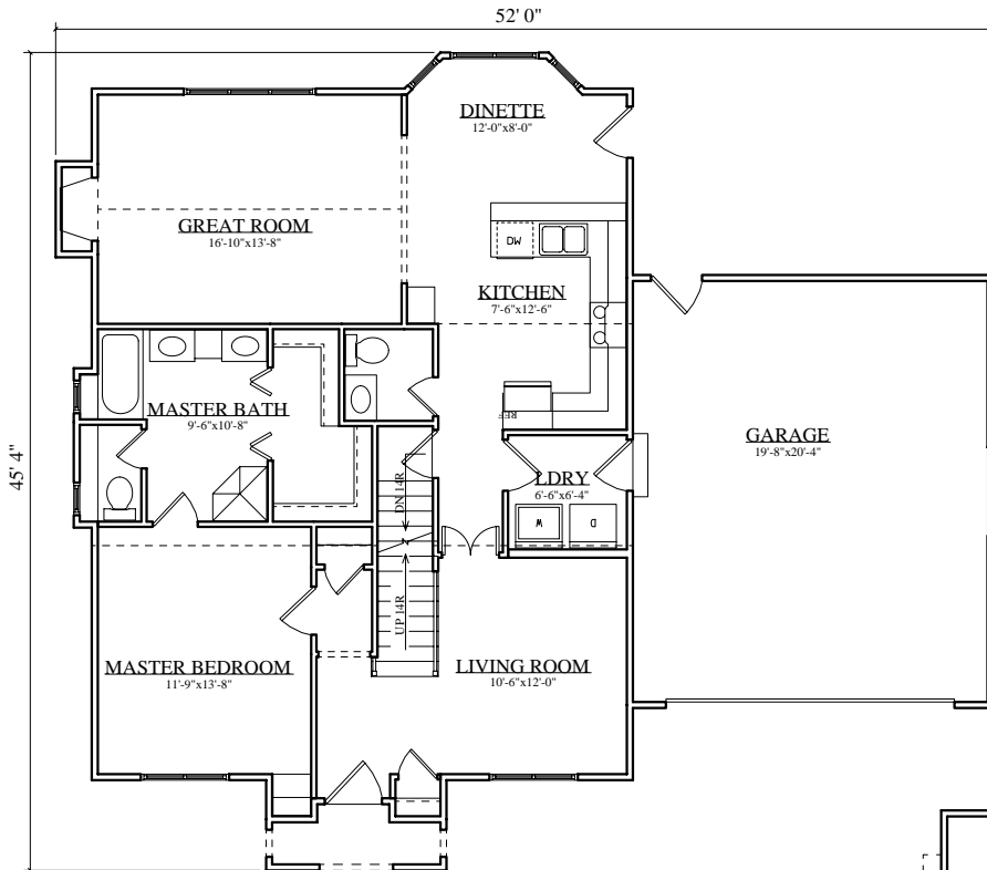
MAIN LEVEL FLOOR PLAN 1,185 SQ. FT.
