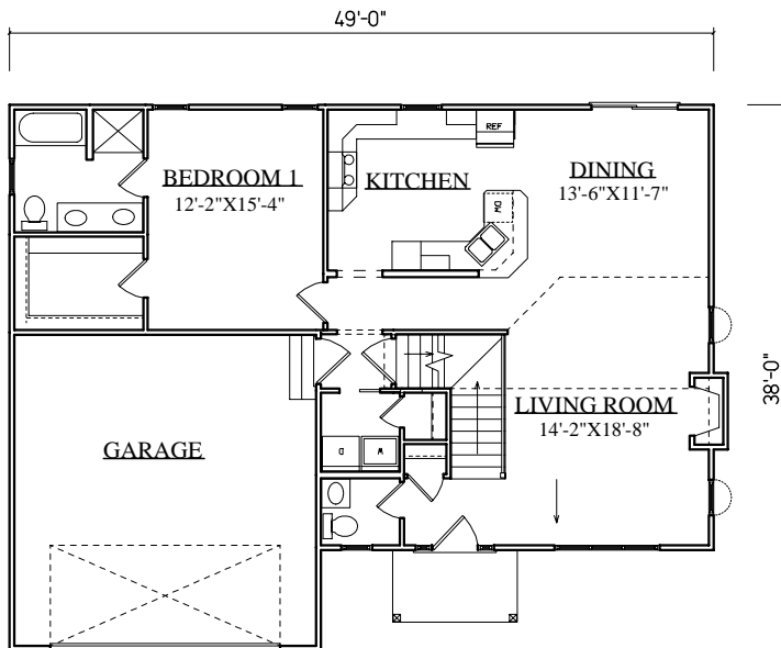
MAIN LEVEL FLOOR PLAN 1,200 SQ. FT.
