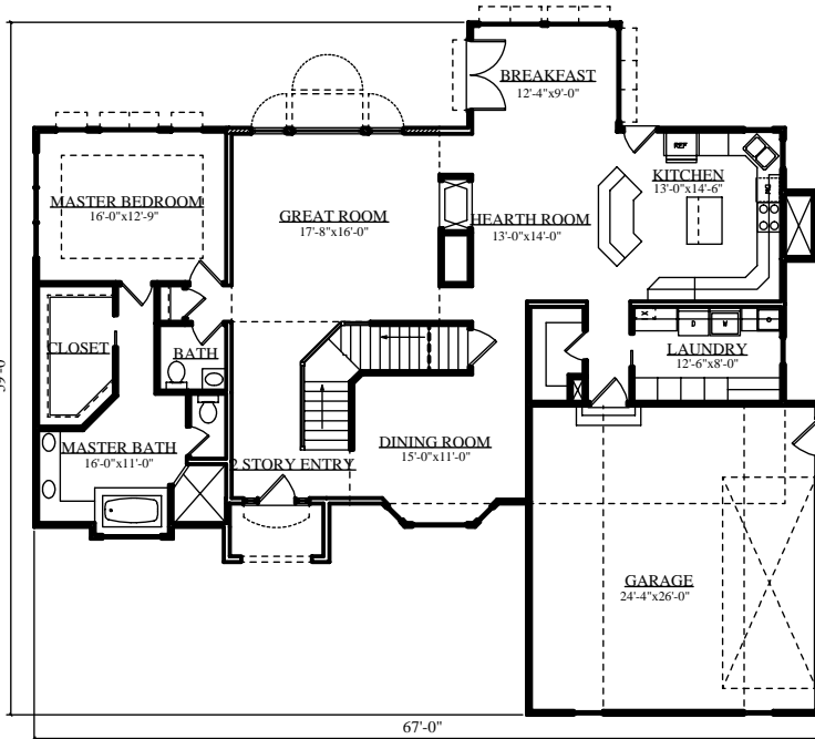
MAIN LEVEL FLOOR PLAN 2,040 SQ. FT.
