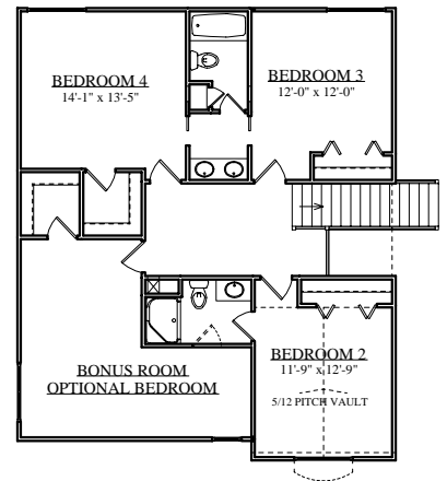
UPPER LEVEL FLOOR PLAN 896 SQ. FT. 1,154 SQ. FT. W/ BONUS
