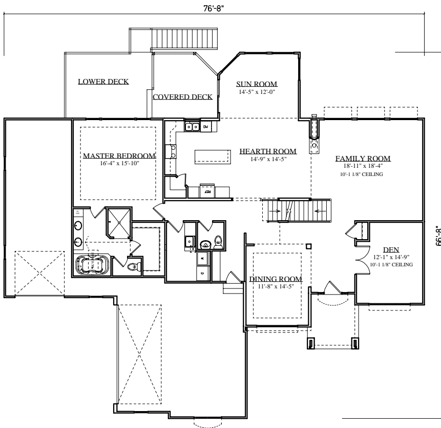
MAIN LEVEL FLOOR PLAN 2,249 SQ. FT.
