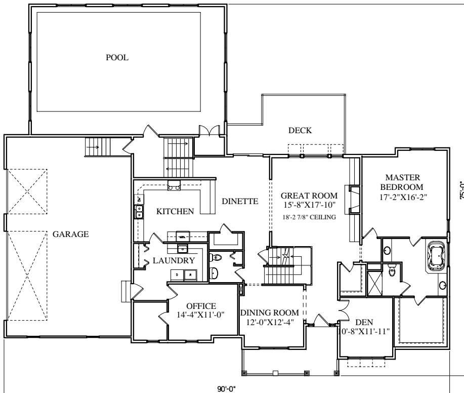
MAIN LEVEL FLOOR PLAN
