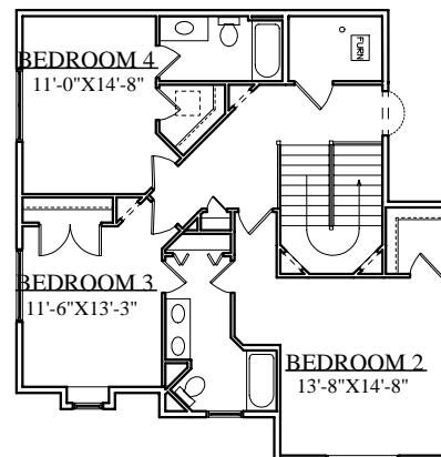
UPPER LEVEL FLOOR PLAN
