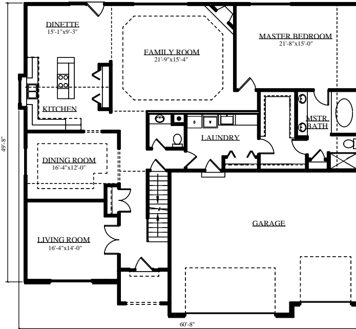
MAIN LEVEL FLOOR PLAN 2,284 SQ. FT.
