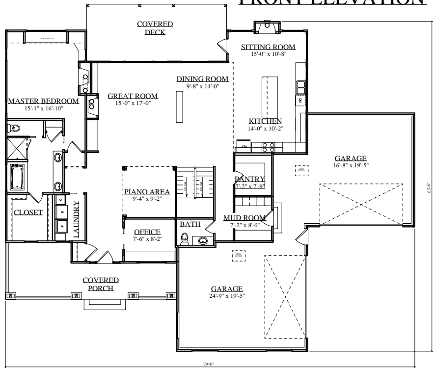
MAIN LEVEL FLOOR PLAN 2,214 SQ. FT.
