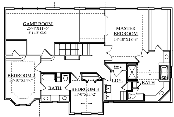
UPPER LEVEL FLOOR PLAN
