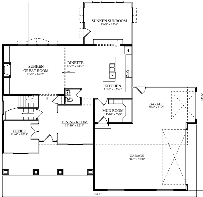
MAIN LEVEL FLOOR PLAN 1,589 SQ. FT.
