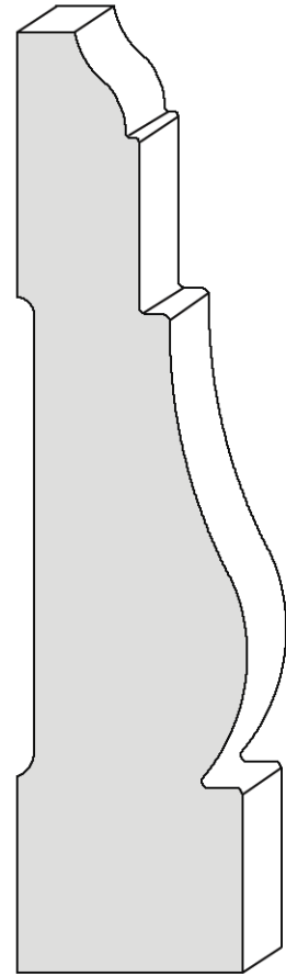
4-7/16" x 1-1/16" BCM054
