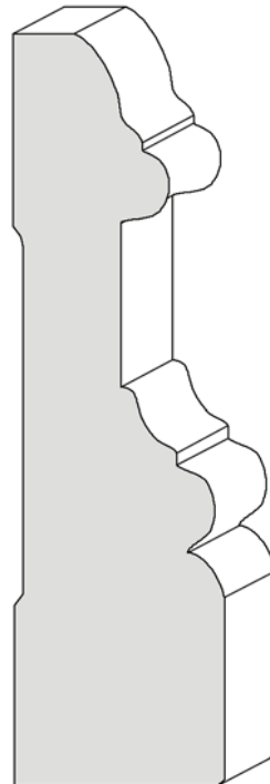
3-1/2" x 1" BCM018
