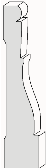
3-7/16" x 3/4" BCM012
