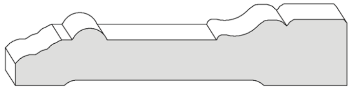
3-1/2" x 11/16" BCM036
