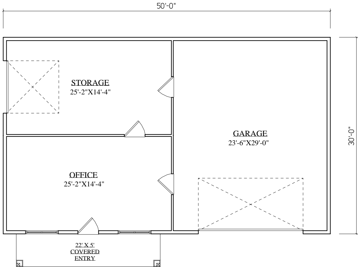
FLOOR PLAN 1,500 SQ. FT.
