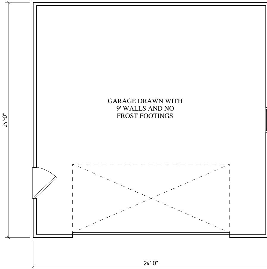
24' X 24' GARAGE FLOOR PLAN 576 SQ. FT.
