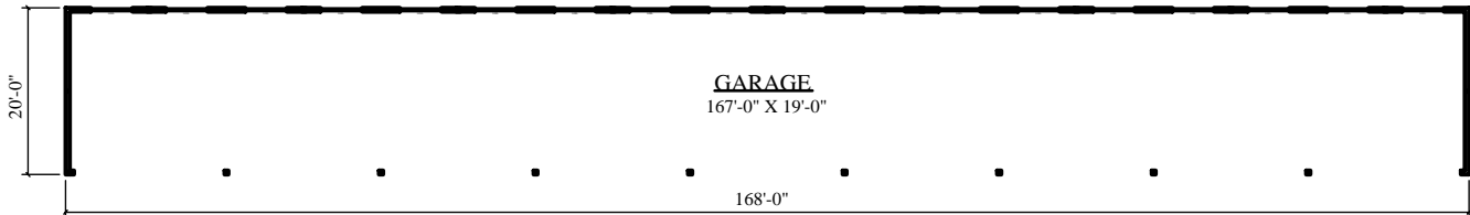
MAIN LEVEL FLOOR PLAN
