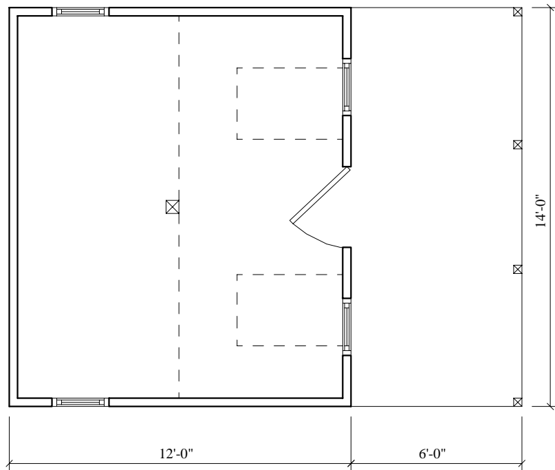
FLOOR PLAN 168 SQ. FT.
