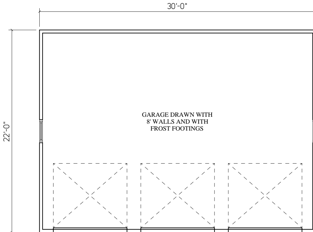
22' X 30' GARAGE FLOOR PLAN 660 SQ. FT.
