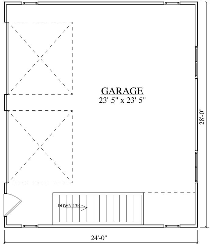
MAIN LEVEL FLOOR PLAN 672 SQ. FT.
