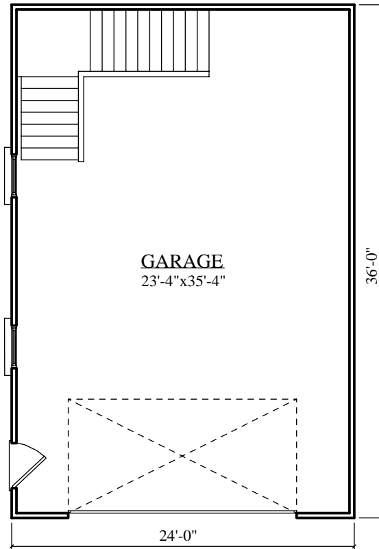
MAIN LEVEL FLOOR PLAN
