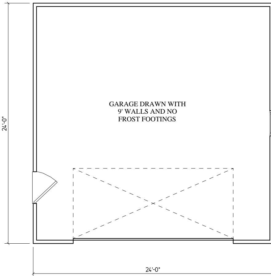
24' X 24' GARAGE FLOOR PLAN
