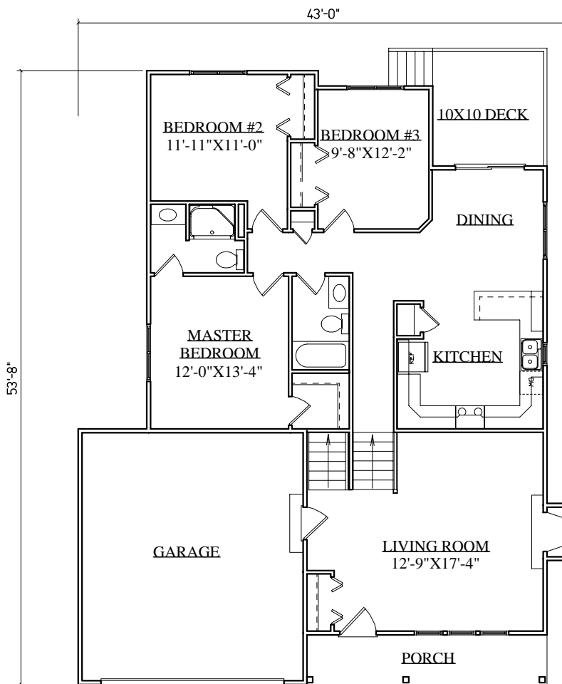
MAIN LEVEL FLOOR PLAN- SPLIT LEVEL
