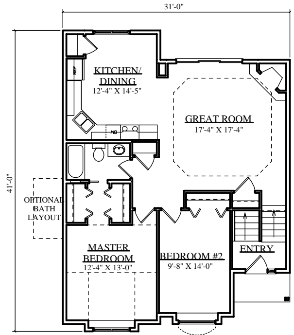
MAIN LEVEL FLOOR PLAN 1,106 SQ. FT. 1,139 SQ. FT. W/OPTIONAL BATH
