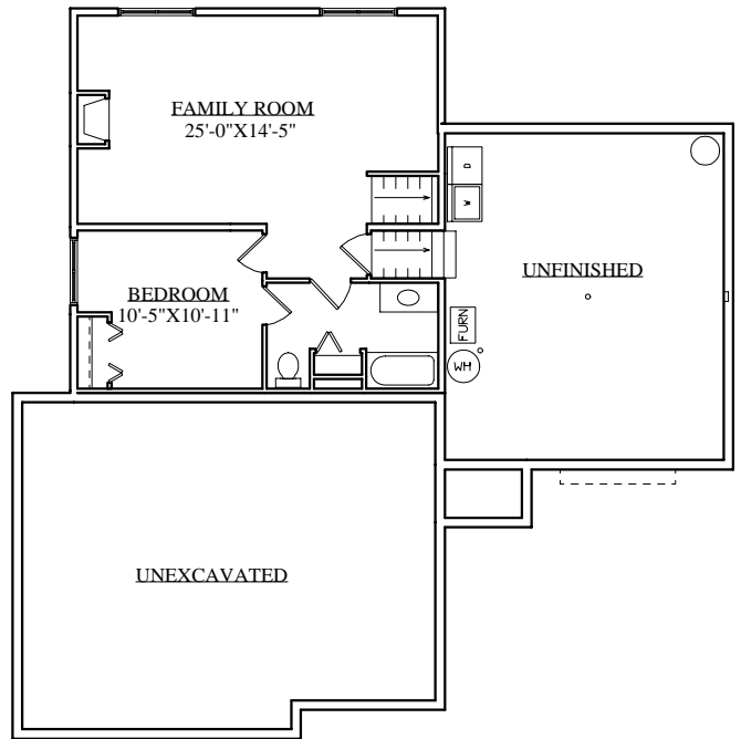
BASEMENT FLOOR PLAN 702 SQ. FT. FINISHED
