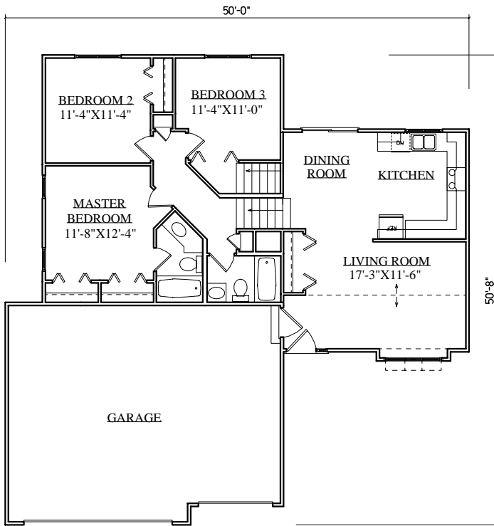
MAIN LEVEL FLOOR PLAN 1,191 SQ. FT.
