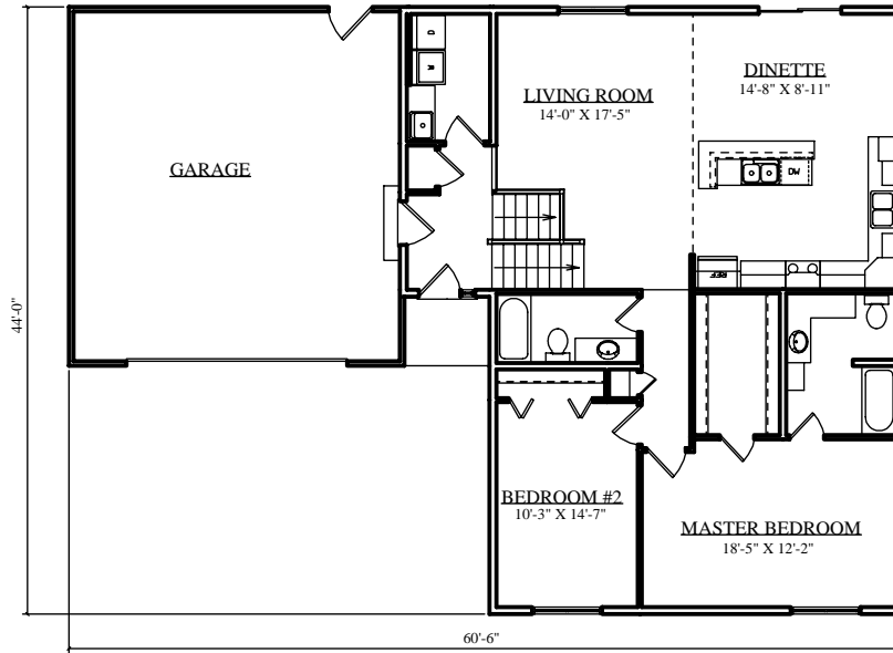
MAIN LEVEL FLOOR PLAN X,XXX SQ. FT.
