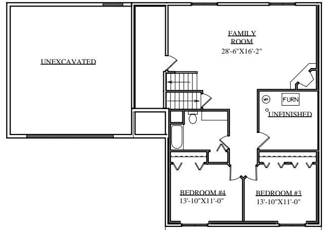
BASEMENT FLOOR PLAN 1,076 SQ. FT. FINISHED
